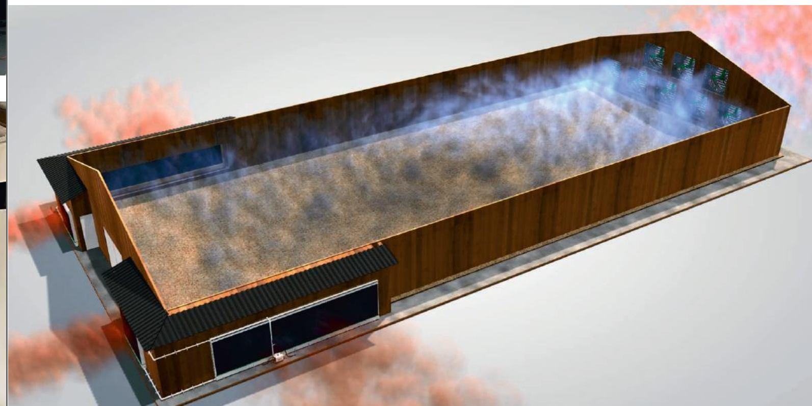
Tunnel ventilation
