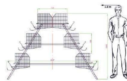
90/96 CAGE
